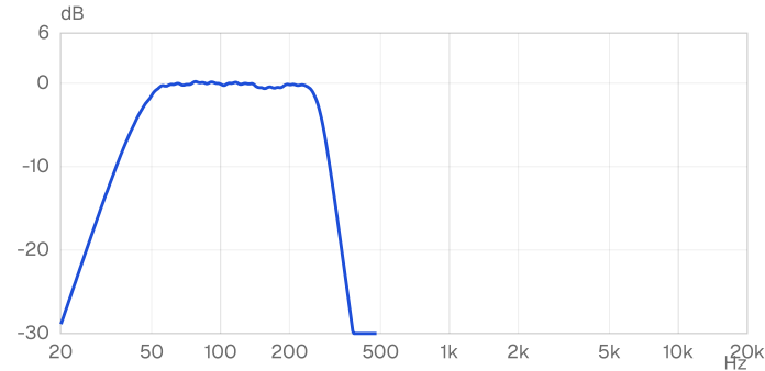
Frequency response: 35 Hz to 300 Hz (-10 dB) · 1/24-octave smoothed
