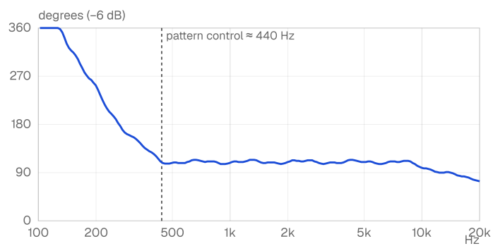
-6 dB horizontal beamwidth: 110° nominal
