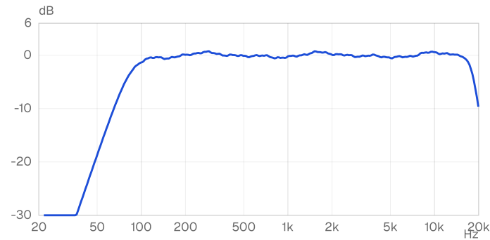
Frequency response: 65 Hz to 20 kHz (-10 dB) · 1/24-octave smoothed
