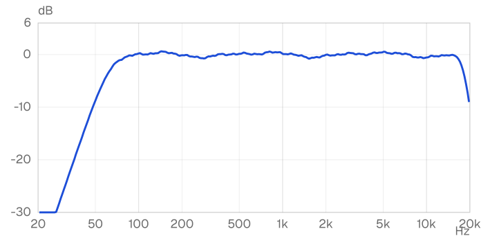
Frequency response: 48 Hz to 20 kHz (-10 dB) · 1/24-octave smoothed
