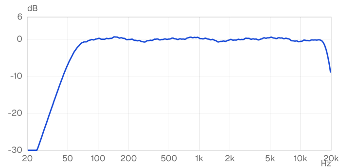
Frequency response: 45 Hz to 20 kHz (-10 dB) · 1/24-octave smoothed
