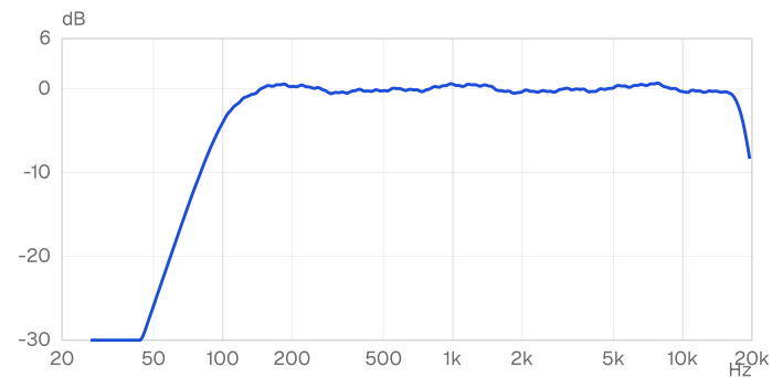
Frequency response: 80 Hz to 20 kHz (-10 dB) · 1/24-octave smoothed
