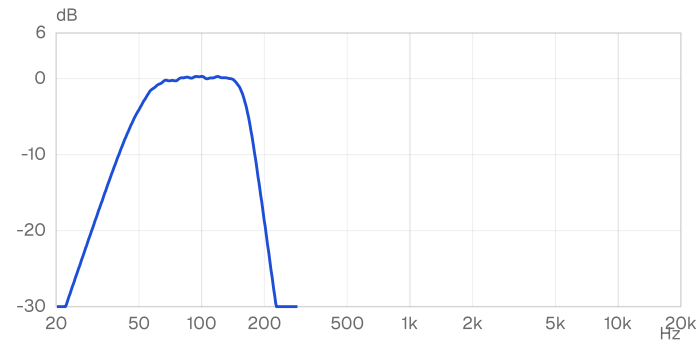
Frequency response: 40 Hz to 180 Hz (-10 dB) · 1/24-octave smoothed
