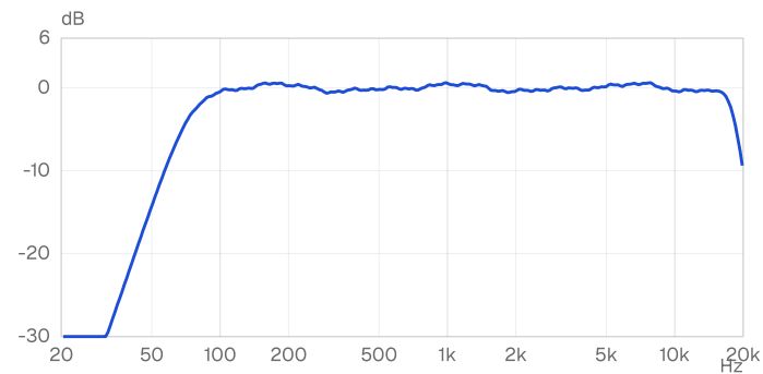
Frequency response: 57 Hz to 20 kHz (-10 dB) · 1/24-octave smoothed
