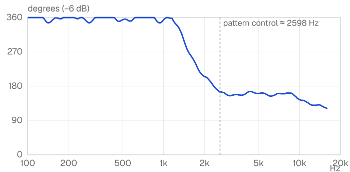
-6 dB horizontal beamwidth: 160° nominal
