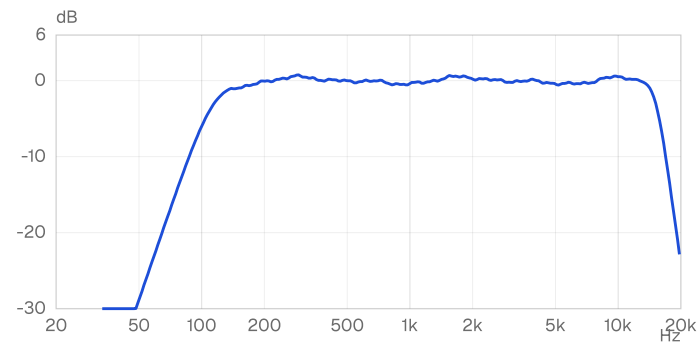
Frequency response: 100 Hz to 16 kHz (-6 dB) · 1/24-octave smoothed
