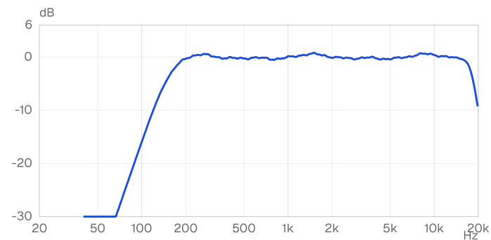
Frequency response: 120 Hz to 20 kHz (-10 dB) · 1/24-octave smoothed
