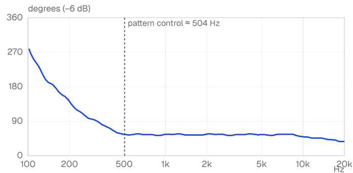
-6 dB horizontal beamwidth: 55° nominal
