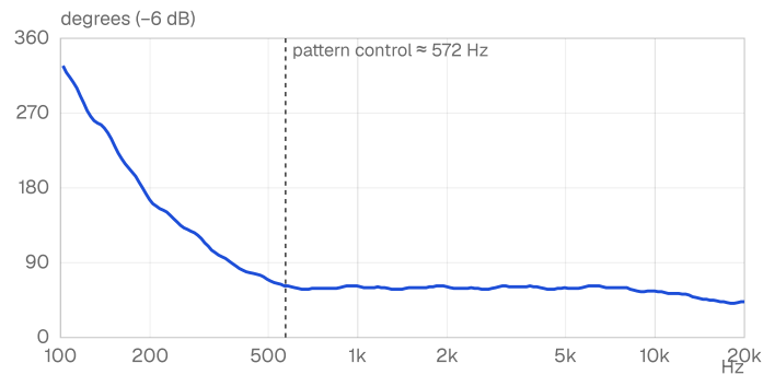
-6 dB horizontal beamwidth: 60° nominal
