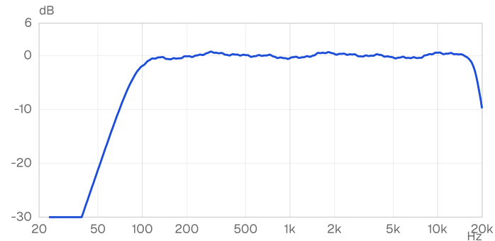
Frequency response: 70 Hz to 20 kHz (-10 dB) · 1/24-octave smoothed
