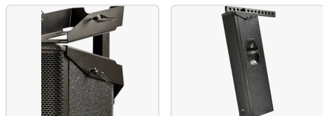
SSOUNDS FLYING BUMPER FOR XTO 8P / 4.6 · PRODUKTANSICHTEN
